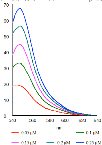
Figure 1 Emission fluorescence spectra of MDA-TBA complex in the range 0.05-0.25 µM MDA ( \lambda_{ex} =530 nm)
